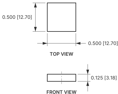
DIMENSIONS Inch [mm] · not to scale
