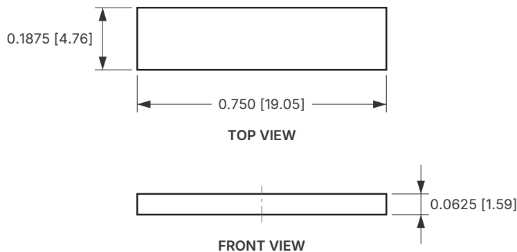
DIMENSIONS Inch [mm] · not to scale
