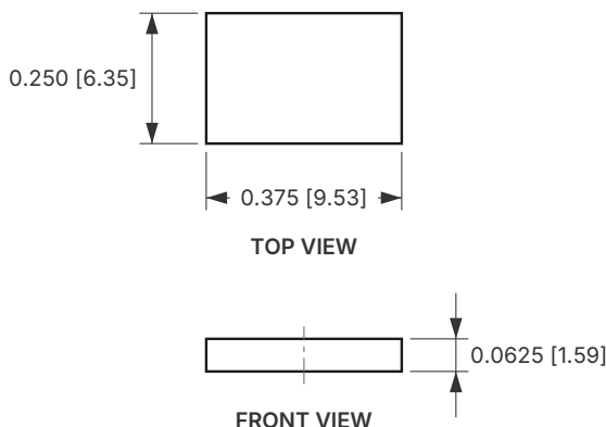
DIMENSIONS Inch [mm] · not to scale
